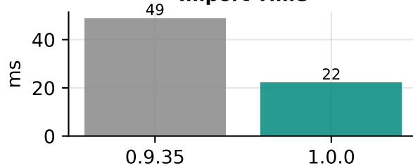
Import Time
