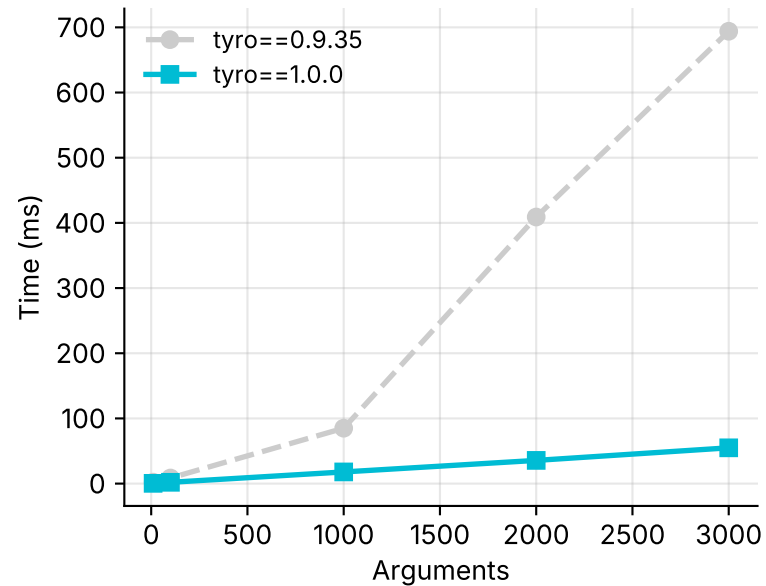
Argument Count vs Runtime
