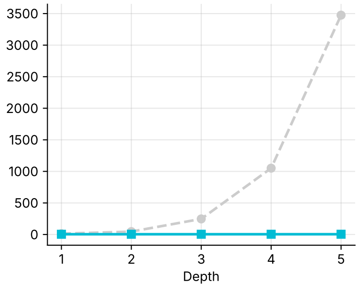
Subcommand Depth vs Runtime
