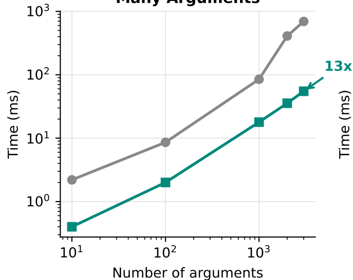
Many Arguments
