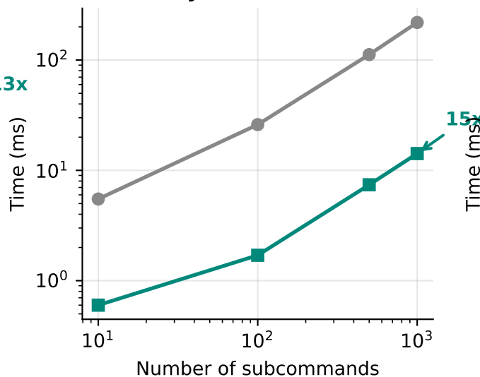
Many Subcommands
