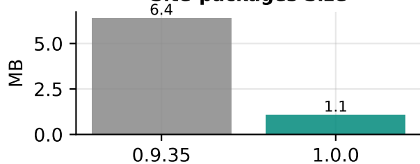
Site-packages Size
