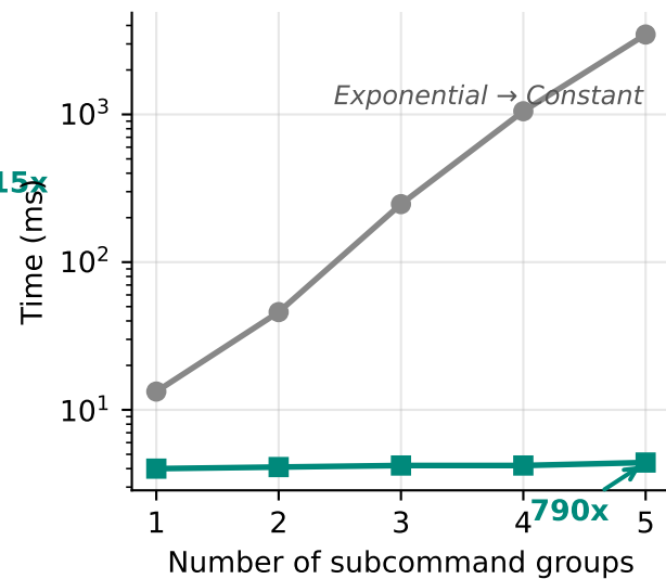
Nested Subcommands
