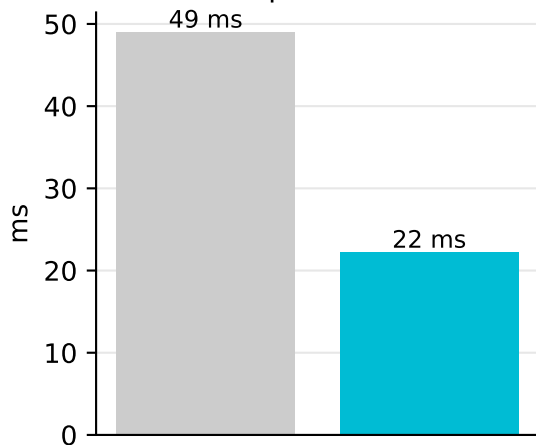
Import time
