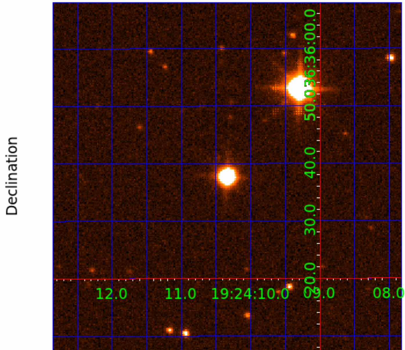
UKIRT Wide Field Camera (WFCAM) infra-red J-band image. The 1' x 1' image is centered on the target (757099).
