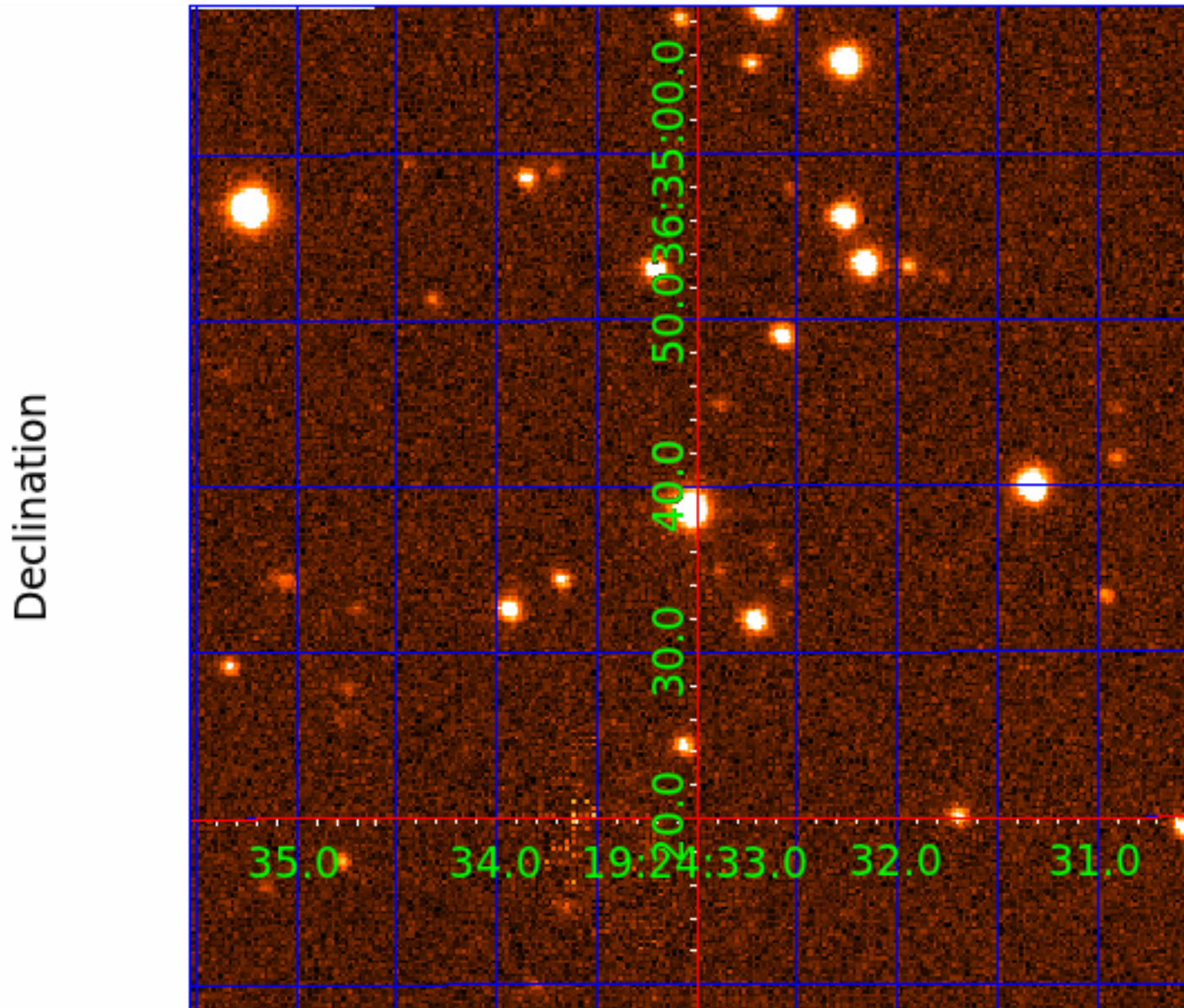
UKIRT Wide Field Camera (WFCAM) infra-red J-band image. The 1' x 1' image is centered on the target (757450).
