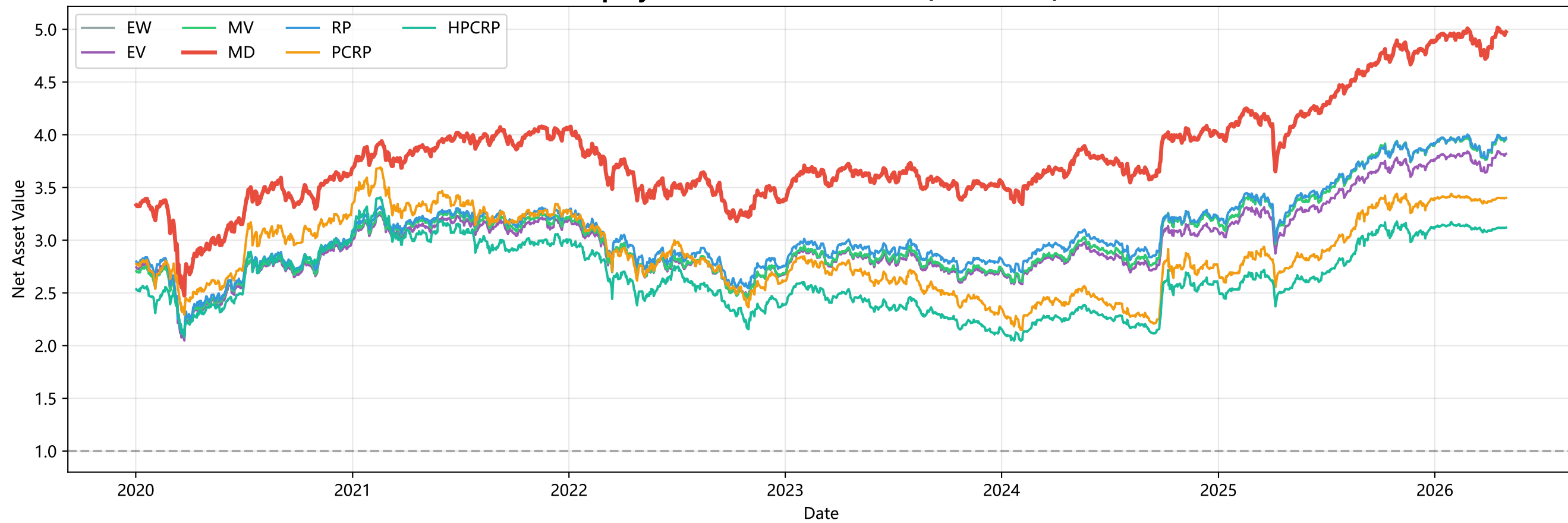
Equity Curves - Recent 5 Years (2020-2026)
