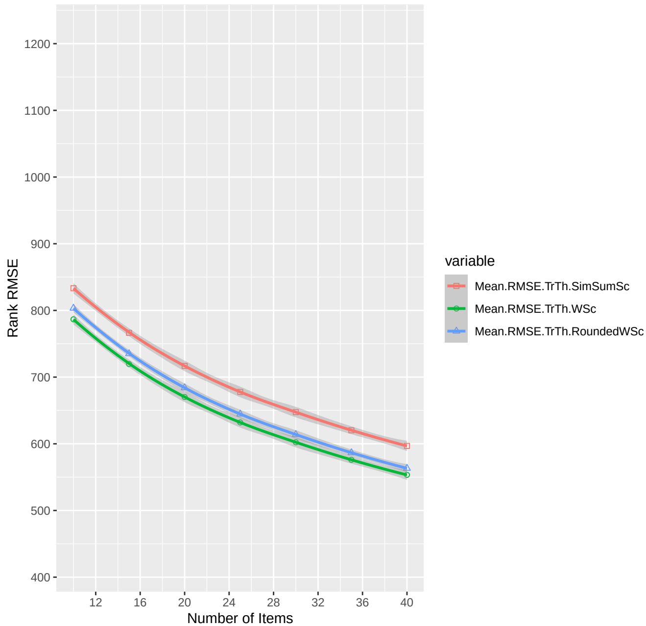
Rank RMSE for reflogist
