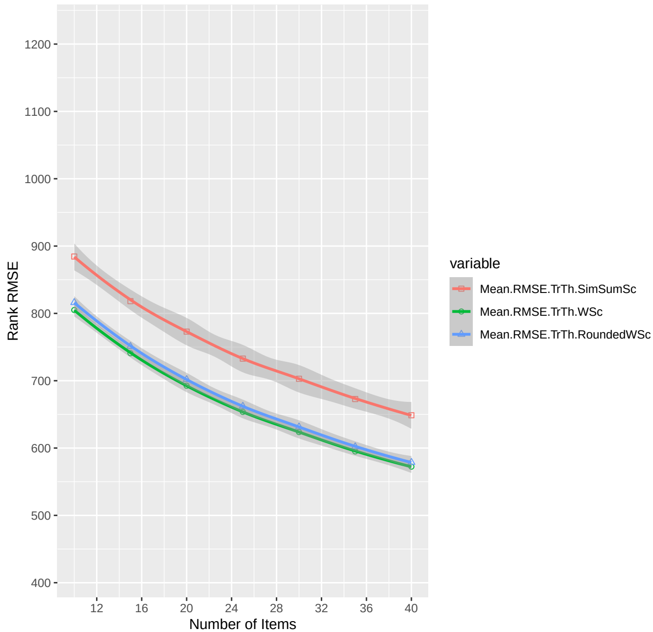
Rank RMSE for noshape
