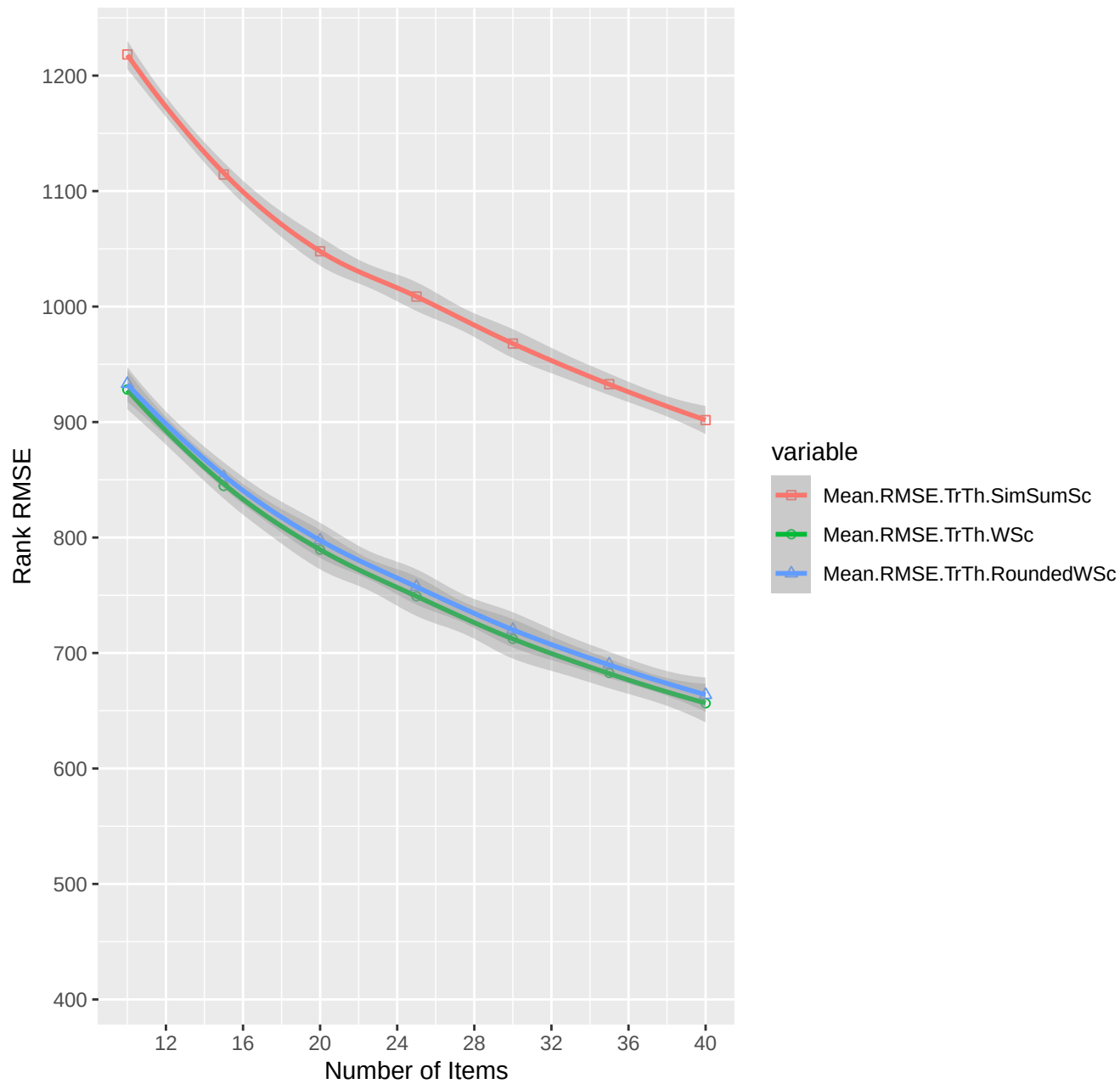
Rank RMSE for neglinear
