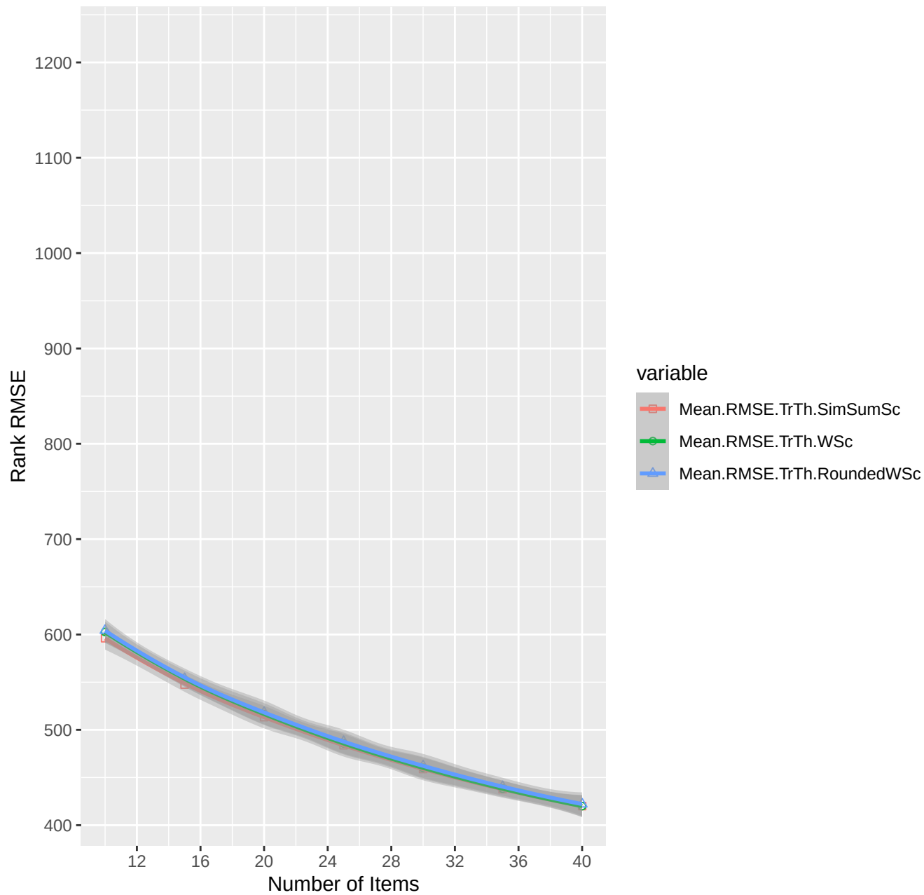
Rank RMSE for leftasym
