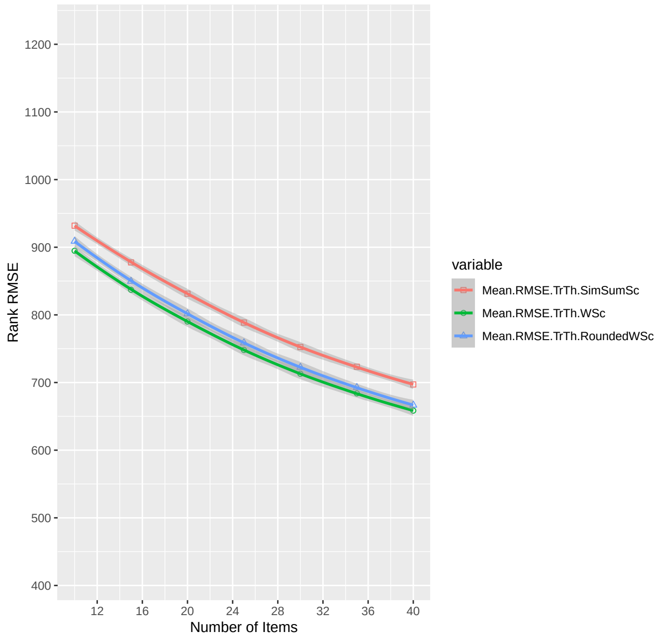
Rank RMSE for expdecay
