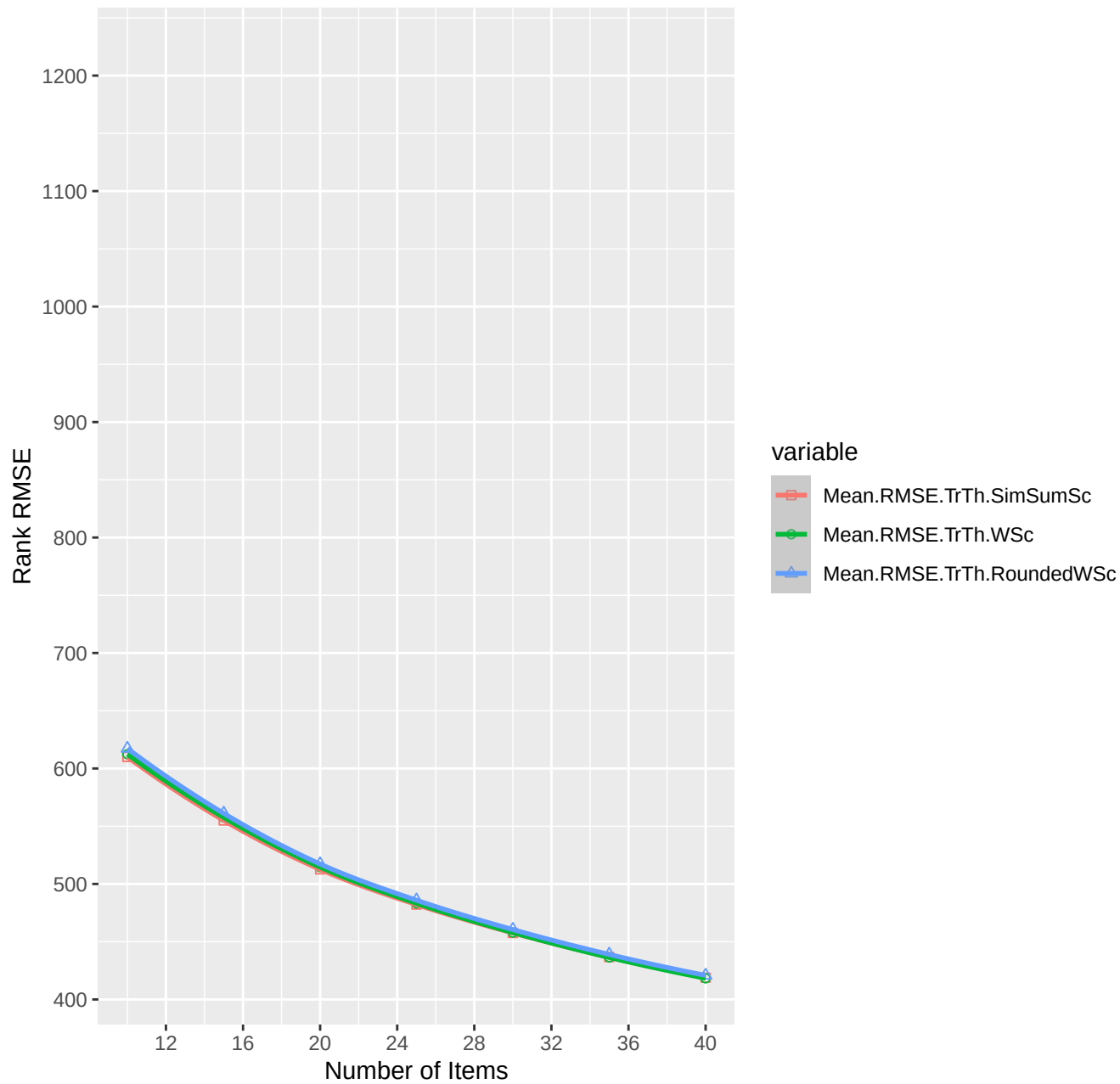
Rank RMSE for rightasym
