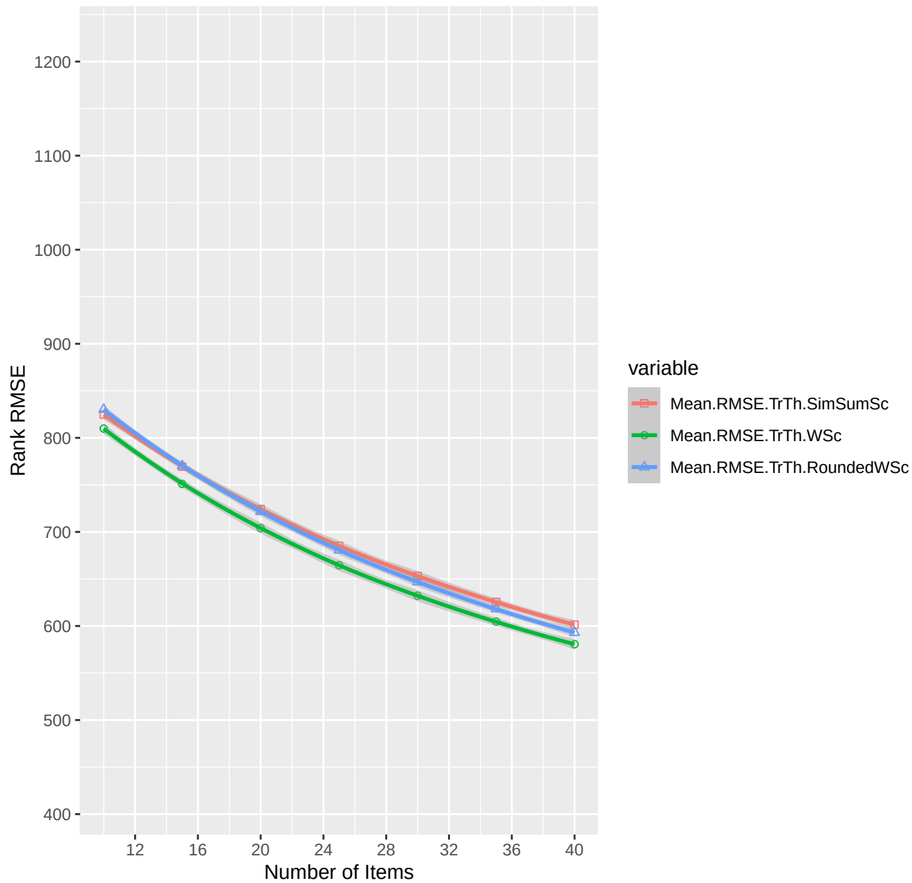
Rank RMSE for invgaussian
