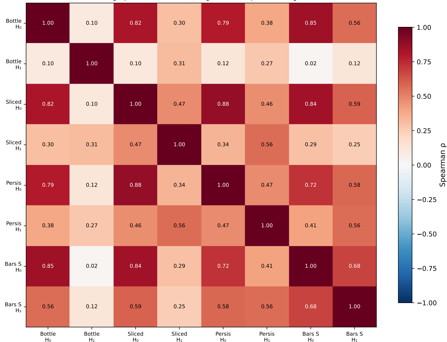
Cross-distance consistency: Spearman \rho between upper triangles (561 pairwise distances per (distance, dim) combination) High \rho = distance notions agree on cell-pair ordering
