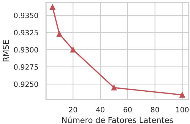
SVD (Model-Based)
