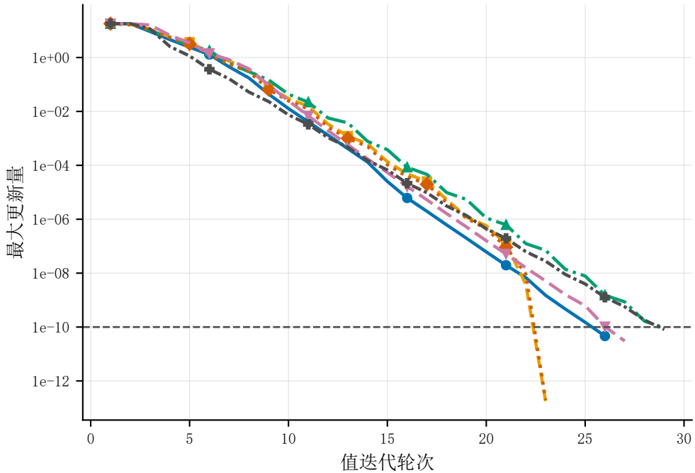
(a) 值迭代收敛
