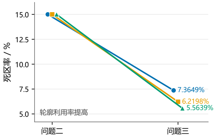
(a) 死区率压缩
