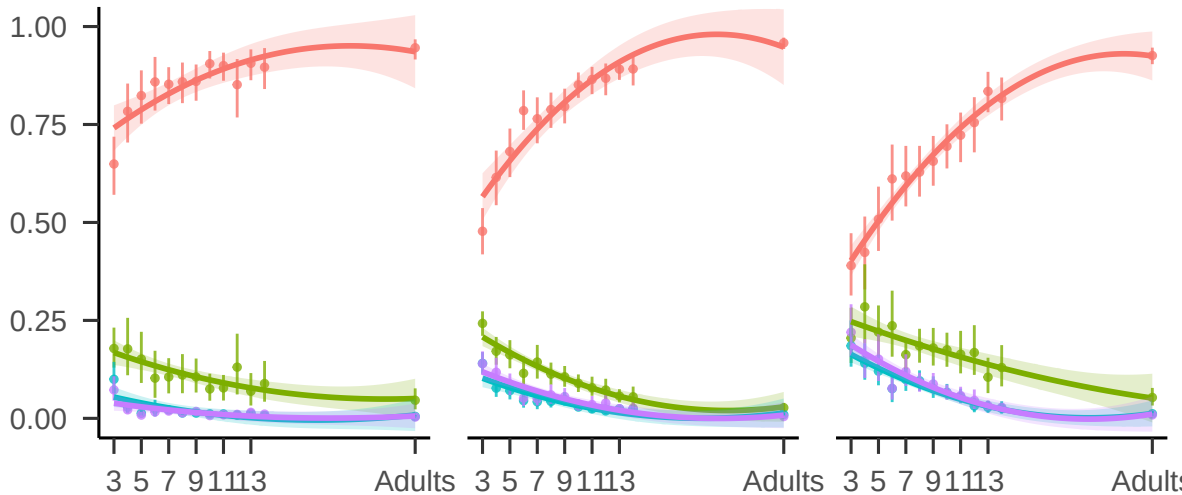
Easy words
