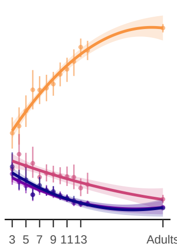
Difficult words
