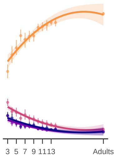
Intermediate words
