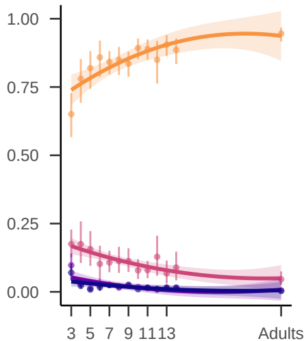
Easy words
