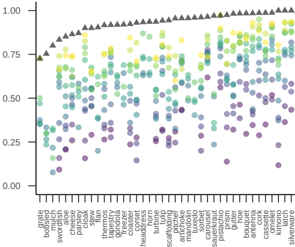
Proportion correct
