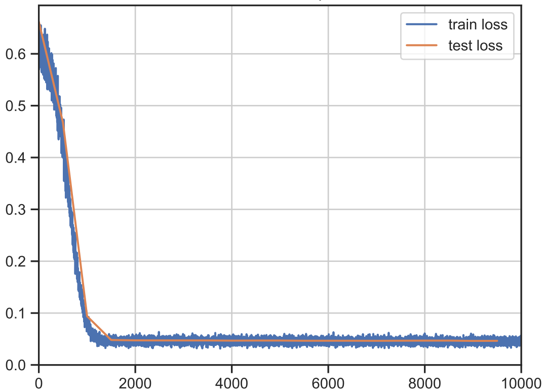
flax.nnx MSE compressor
