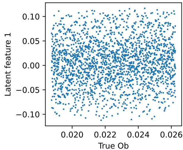
s2MSE_L750_6000N_1500steps_64batch_0.0015lr
