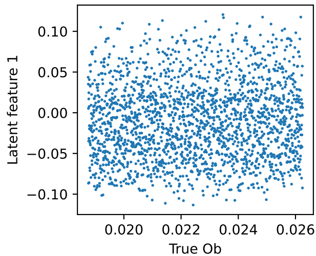
s2MSE_L750_6000N_2000steps_64batch_0.0015lr
