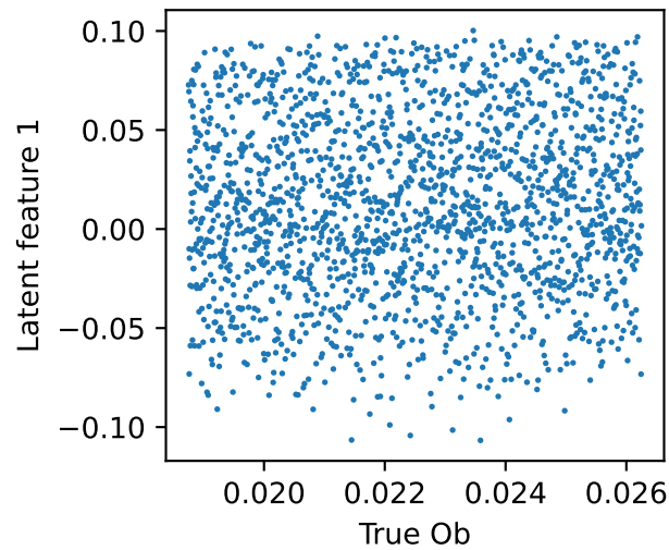
s2MSE_L750_6000N_700steps_128batch_0.005lr
