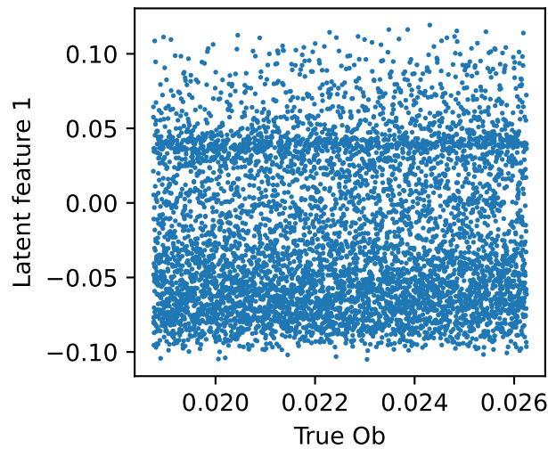
s2MSE_L1500_6000N_1200steps_32batch_0.002lr
