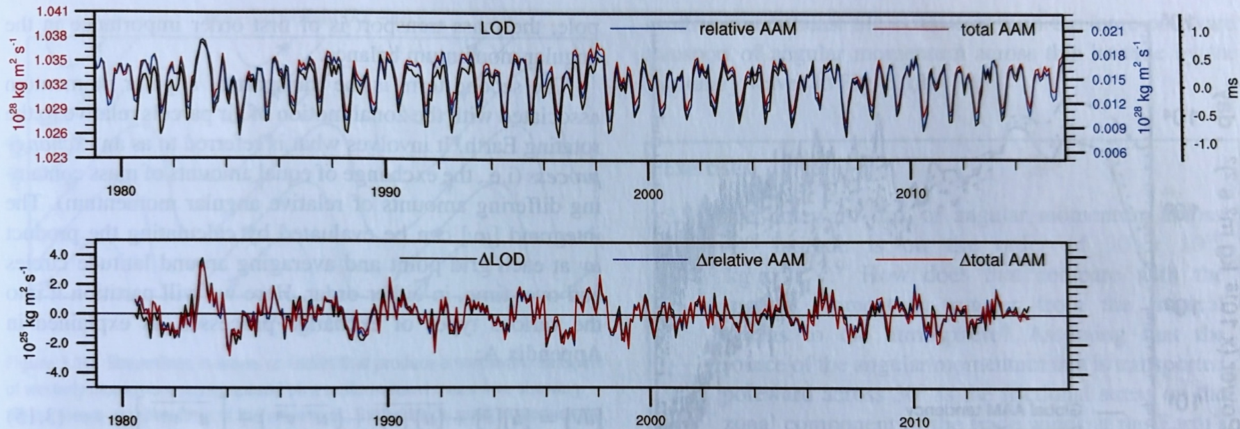
Figure 3.5 (Top) Time series of total and relative atmospheric angular momentum AAM as defined in Eq. (3.6) indicated by the red and blue curves, respectively, together with length of day LOD indicated by the black curve. The interdecadal variability in LOD attributable to motions in the Earth's mantle has been removed and the curve has been scaled in accordance with Eq. (3.7) to make it compatible with the AAM curves. The scales at the left and right are different because the total AAM contains the almost constant solid body rotation component. The LOD scale in units of milliseconds is also included at the far right. (Bottom) The corresponding anomalies with respect to the seasonally varying climatological means. Courtesy of Ying Li.
