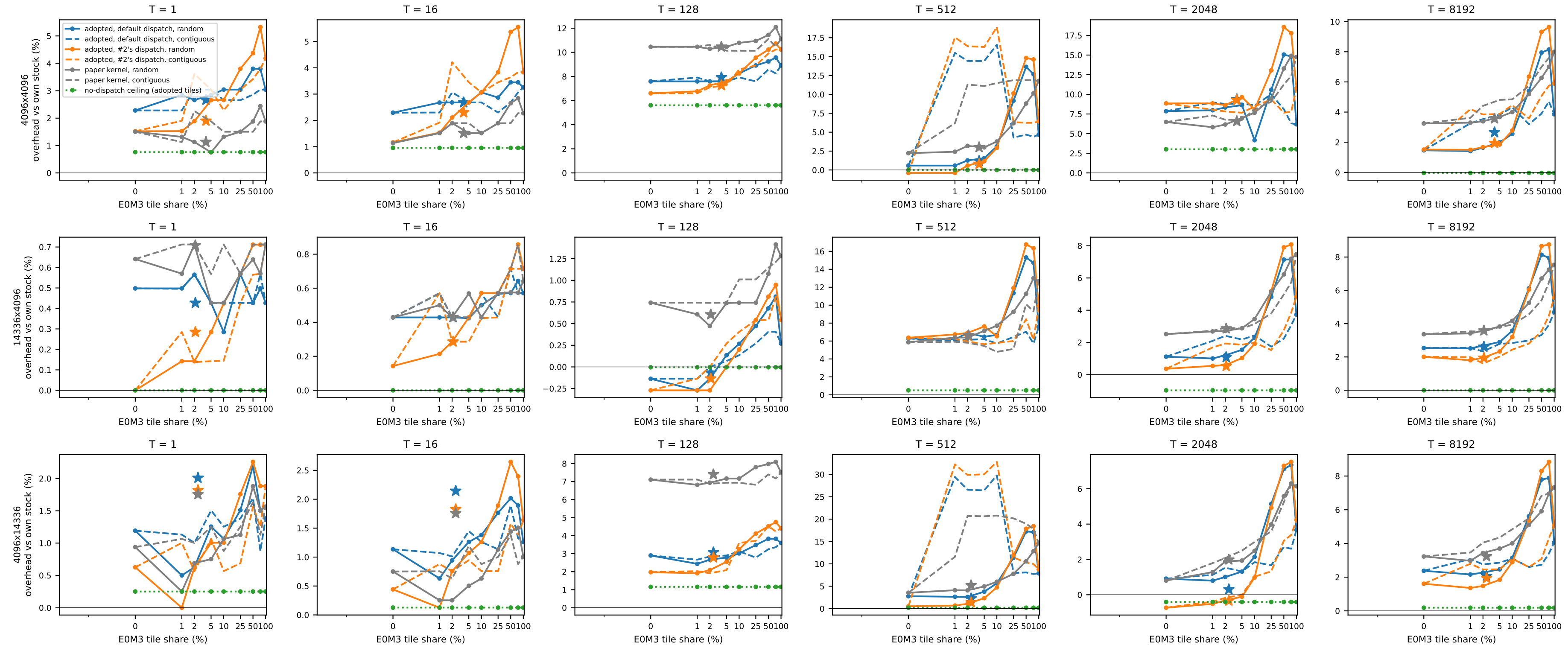
GEMM overhead vs E0M3 tile share (stars: real TM-OPT+TC 16x64 map, typical module)
