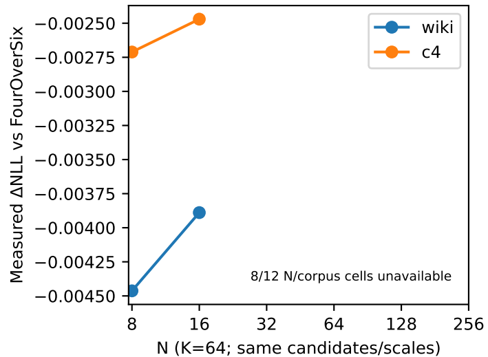
mistral7b seed0 joint k=3
