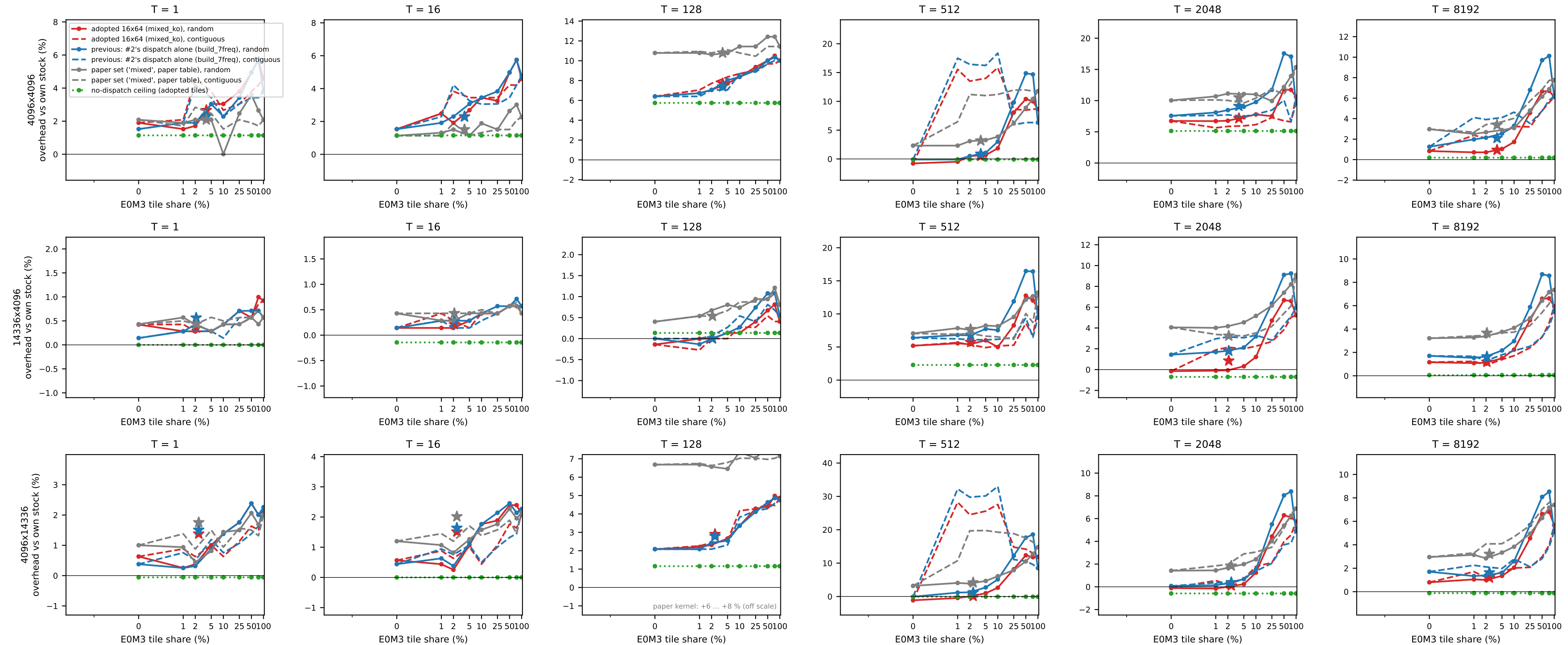
16x64: GEMM overhead vs EOM3 tile share (stars: real TM-OPT+TC 16x64 map, typical module)
