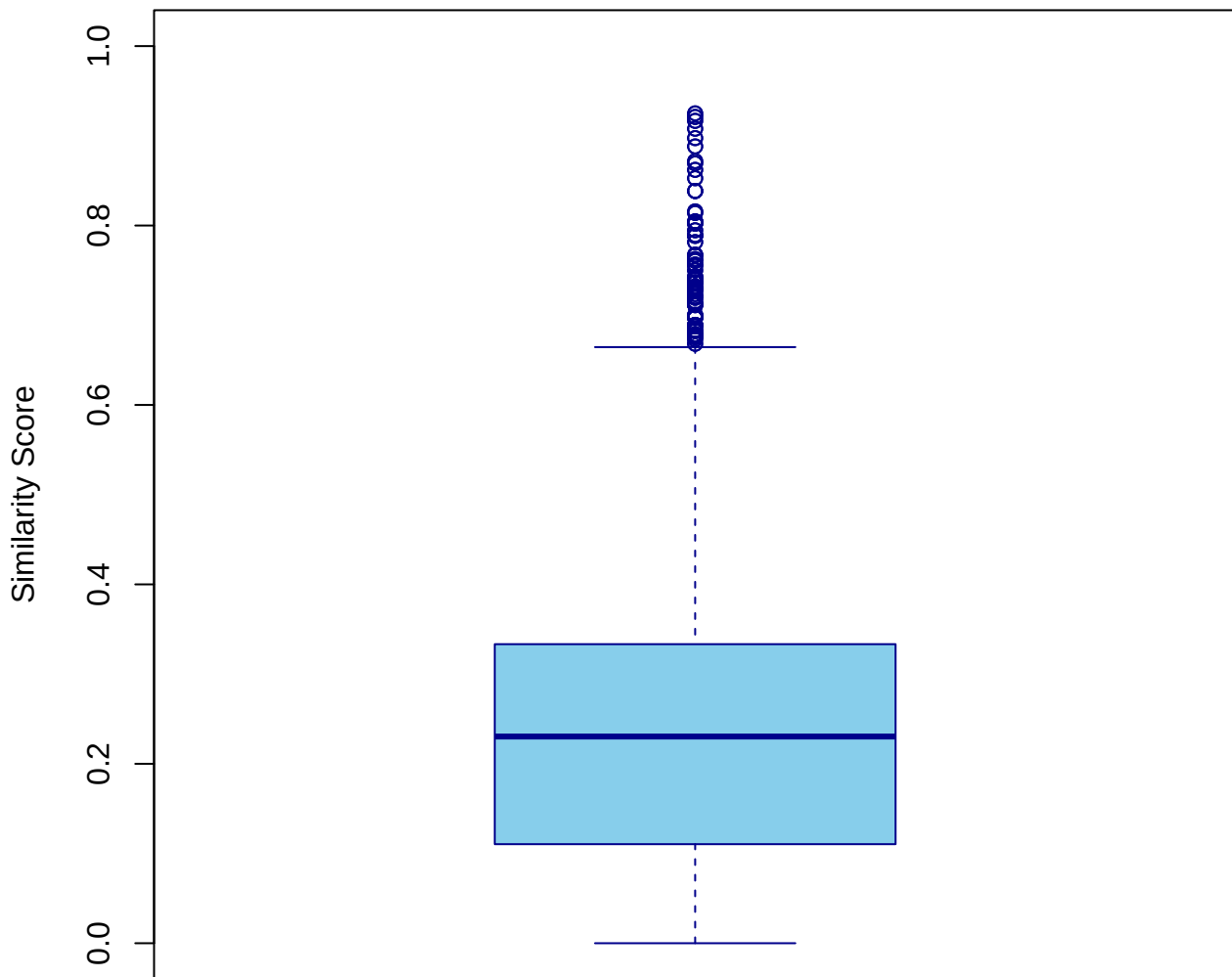
levenshtein Similarity Score Distribution
