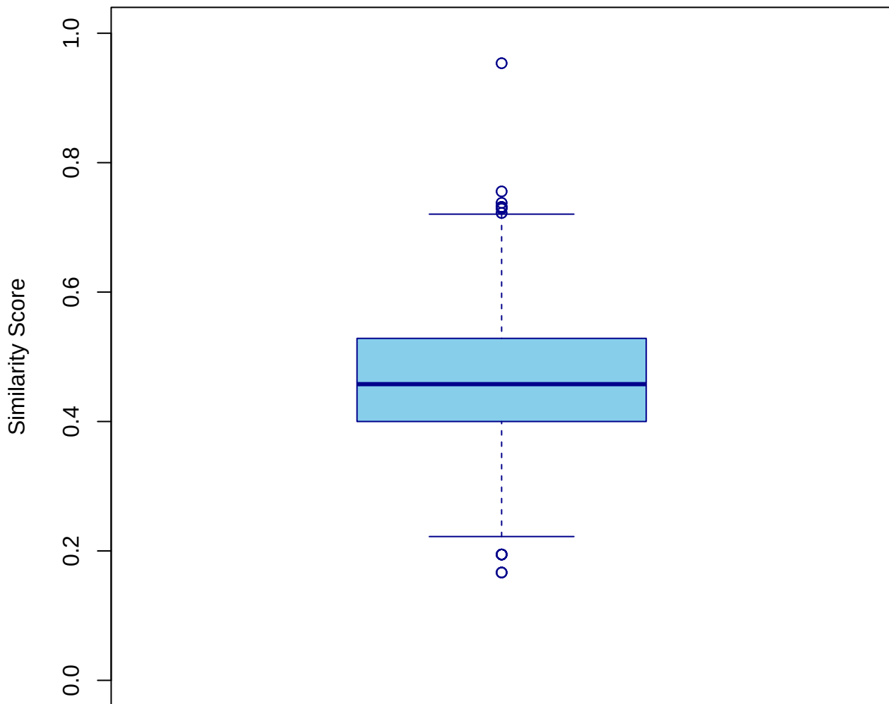
winnowing Similarity Score Distribution
