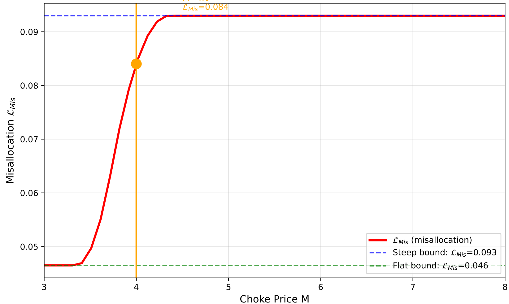
Misallocation vs Choke Price (Rationed Allocation)
