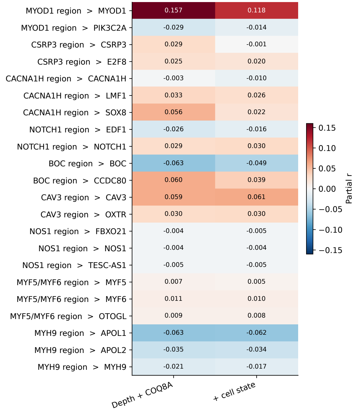
A Peak-RNA partial correlation
