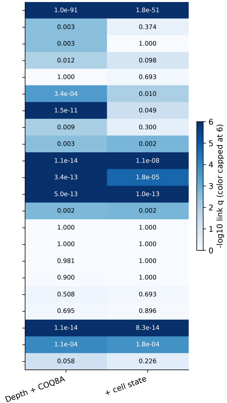
B Peak-RNA evidence
