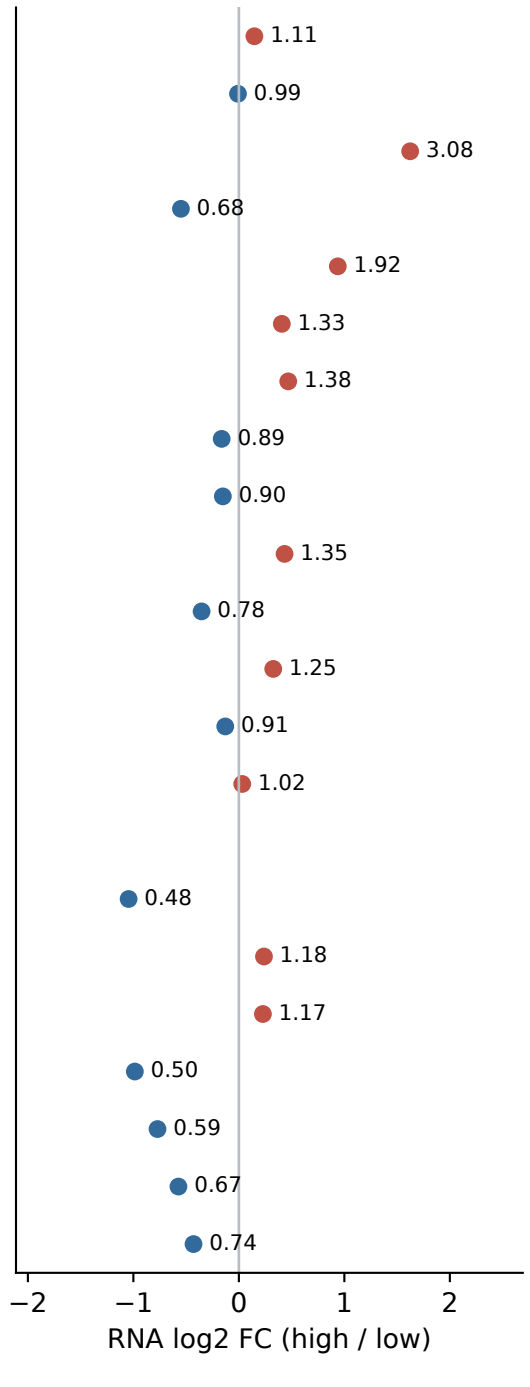
C Same-pair RNA response
