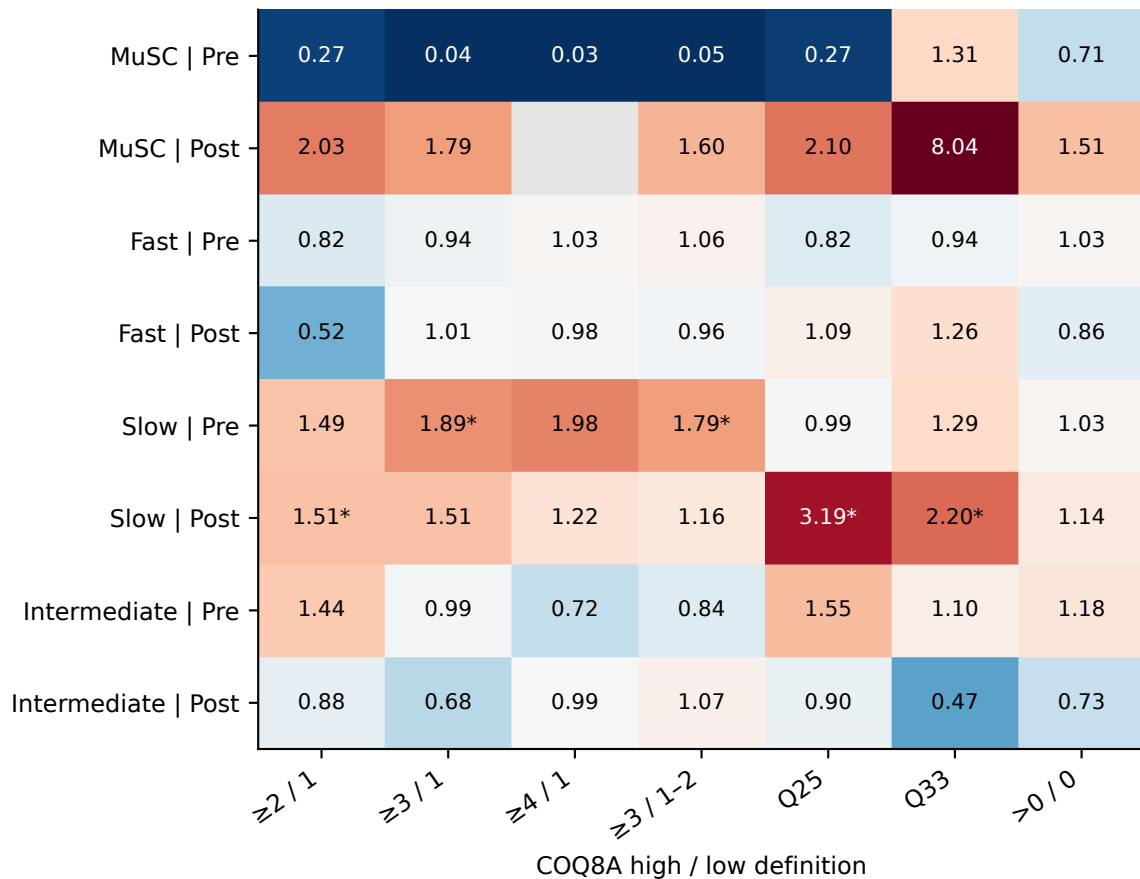
A All eligible nuclei; RNA-depth covariate
