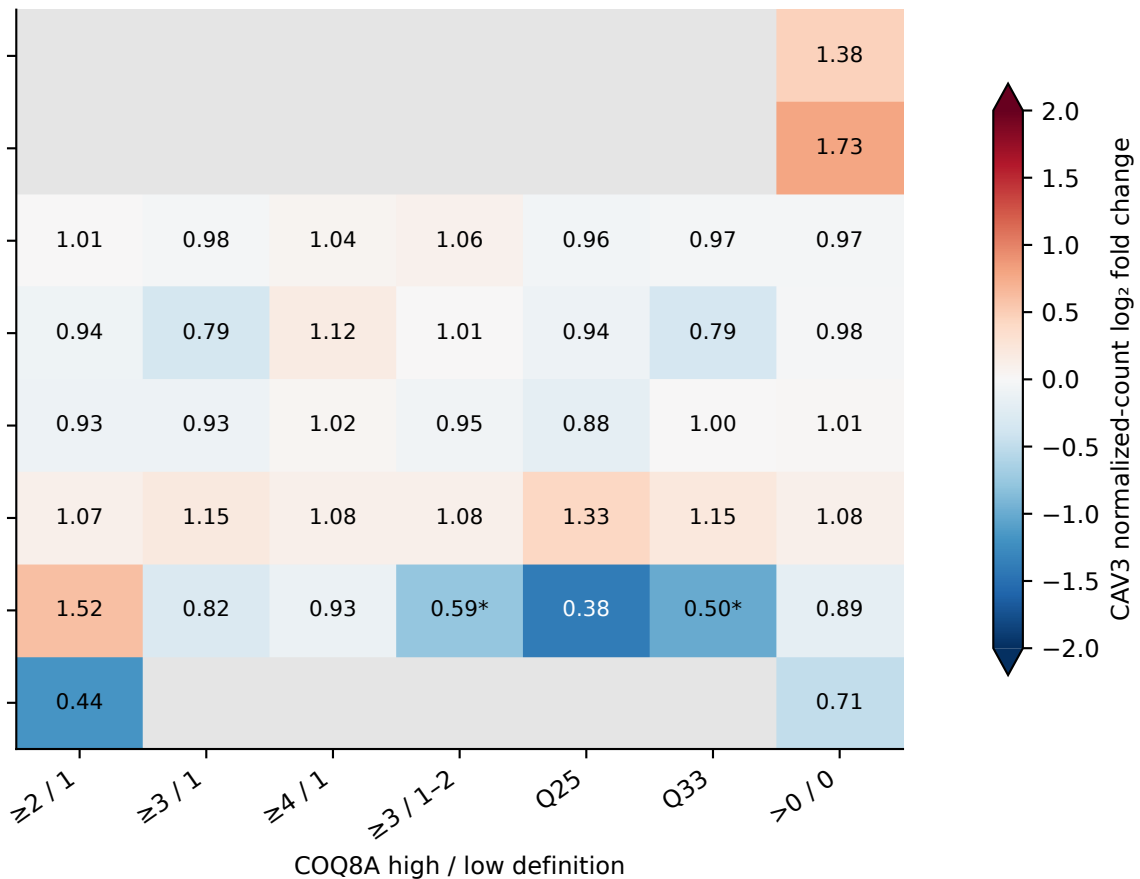
B Depth-matched nuclei; caliper 0.10
