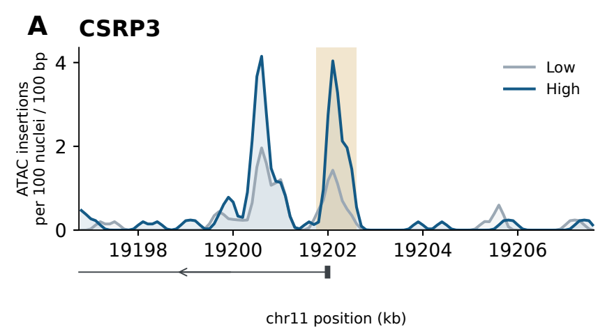
ATAC fragment signal
