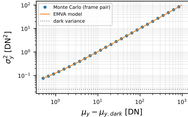
Photon transfer
