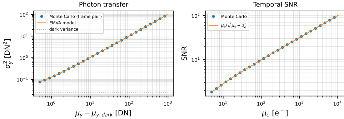
Figure 2. EMVA1288 photon-transfer validation for the iphone_8 recipe. Left: temporal variance versus dark-subtracted mean signal for Monte Carlo frame pairs (markers) and the analytic model (line); the gain fit uses levels up to 70% of full well. Right: temporal SNR versus mean electrons.
