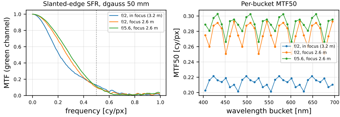
Figure 3. Slanted-edge MTF through the traced 50 mm double-Gauss lens. Left: green-channel MTF for three aperture/focus settings (dotted line: Nyquist). Right: MTF50 computed separately in each spectral bucket of the same renders; the periodic ripple is unexplained (see text).
