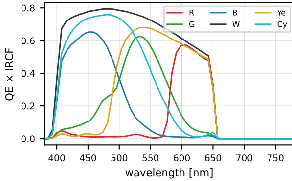
Figure 4. Generic QE \times IRCF curves shipped in spectra/QE/interpolated/ and used for the CFA study (W: unfiltered monochrome QE).
