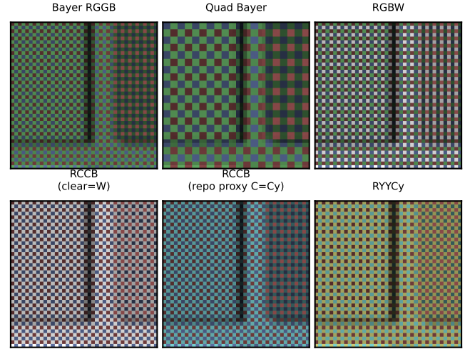
Figure 5. Raw mosaics computed from one spectral render (D65) at the corner of patches 14, 15, 20 and 21, each pixel tinted by its filter. Only Bayer is sampled by the pipeline itself; the other layouts are produced by fig_cfa.py from the same spectral buckets.
