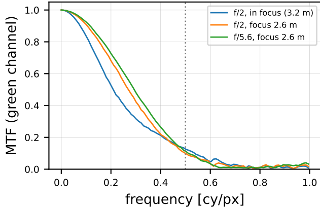
Slanted-edge SFR, dgauss 50 mm
