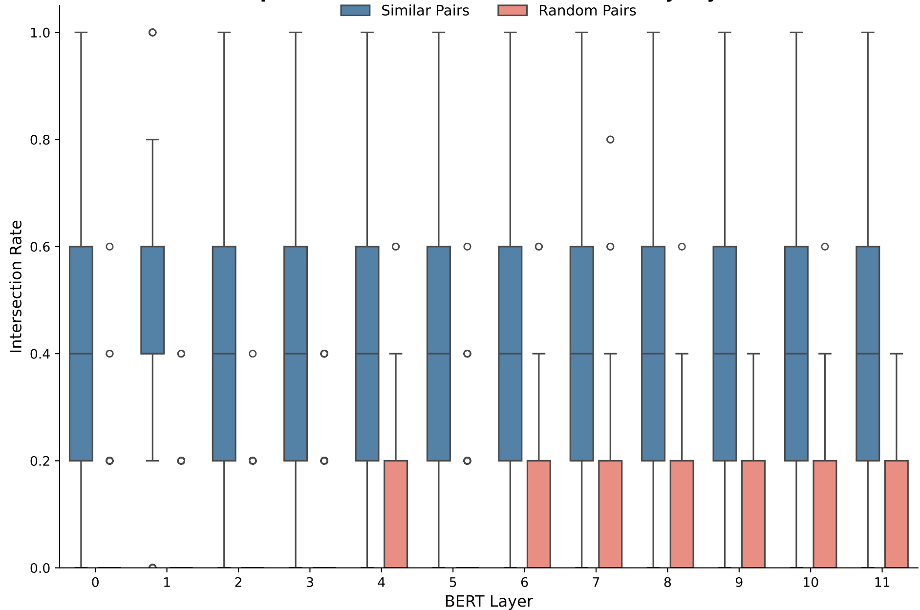
Top-5 Neuron Intersection Distributions by Layer
