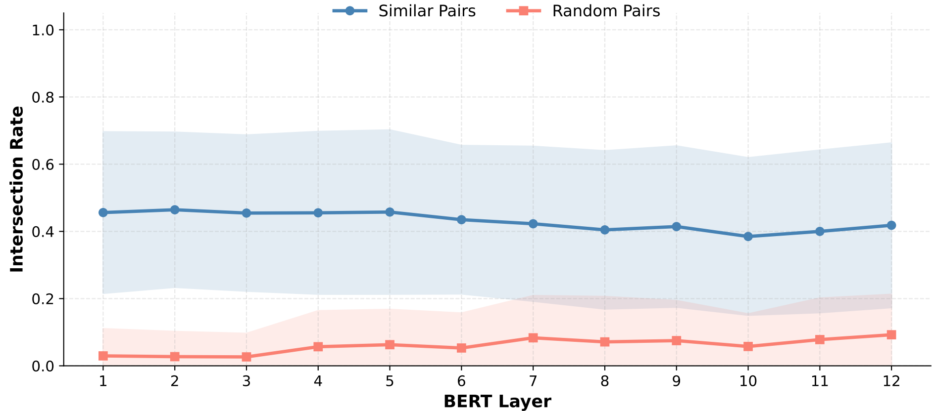
Top-5 Neuron Intersection Rate by Layer
