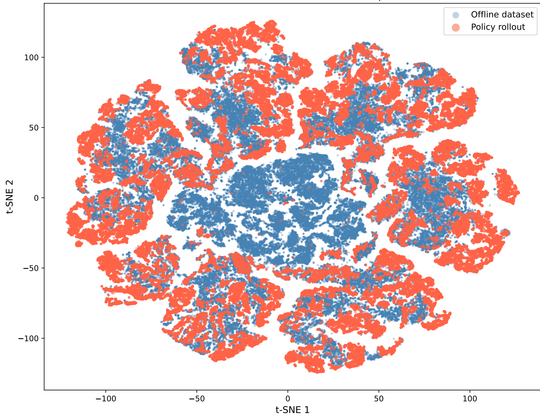
COMBO-RealNVP (halfcheetah-medium-expert-v2)
