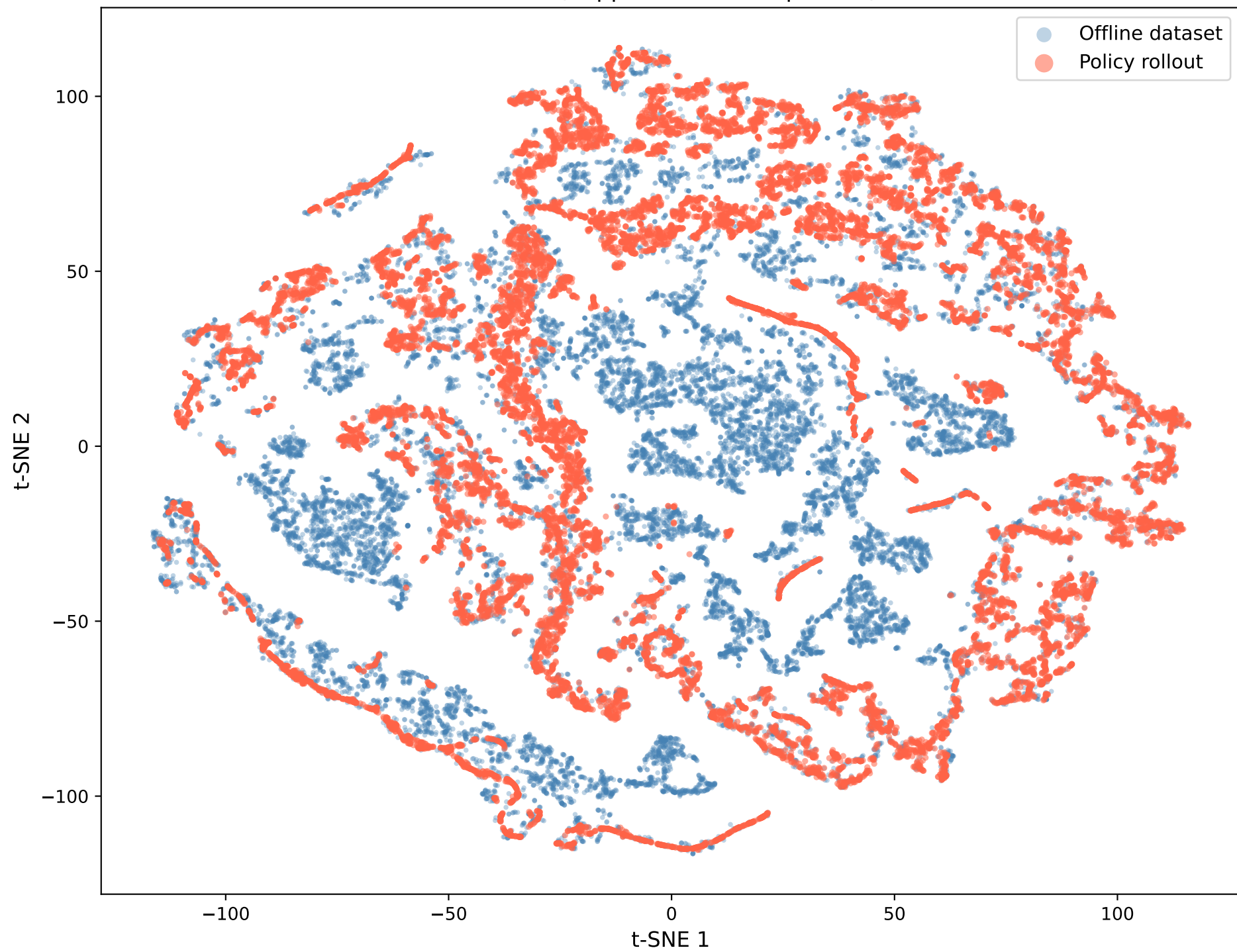
COMBO (hopper-medium-expert-v2)
