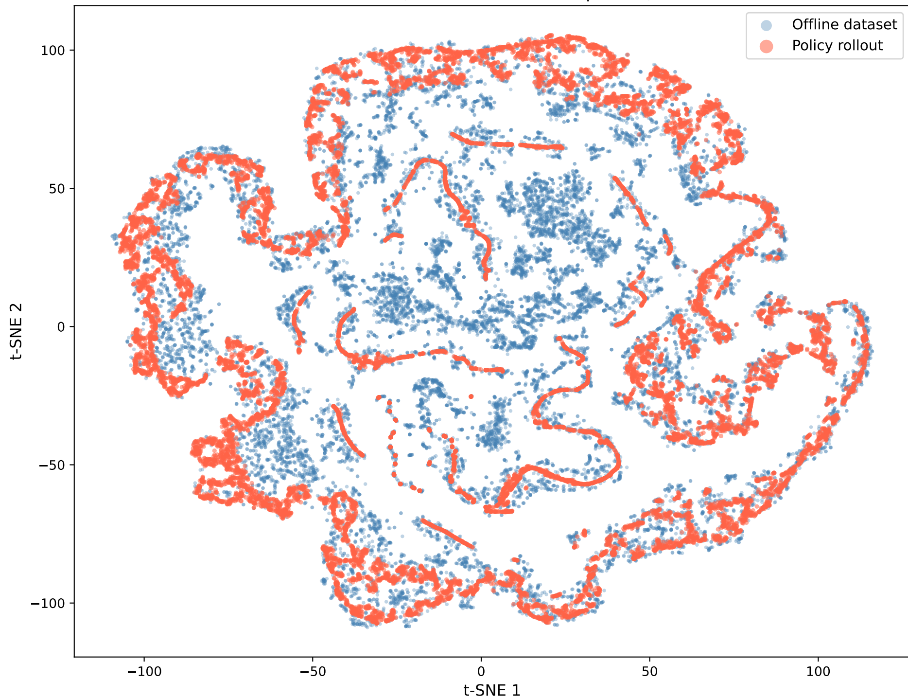
COMBO (walker2d-medium-expert-v2)
