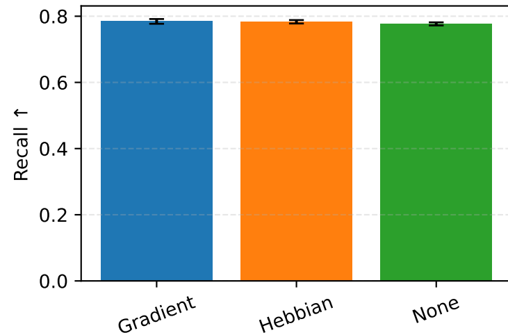
Copying (delay 20)
