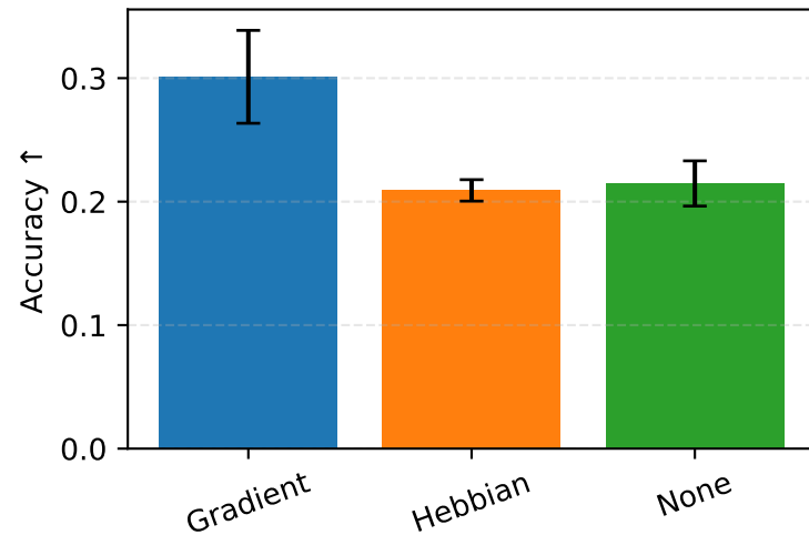
Omniglot 5-way/1-shot
