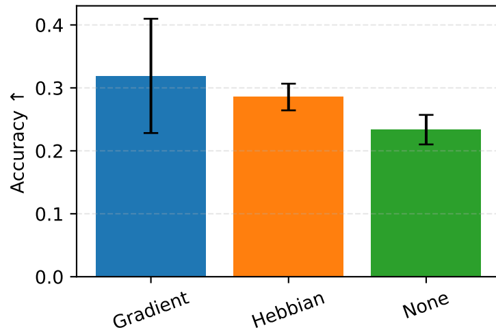
CIFAR-FS 5-way/1-shot
