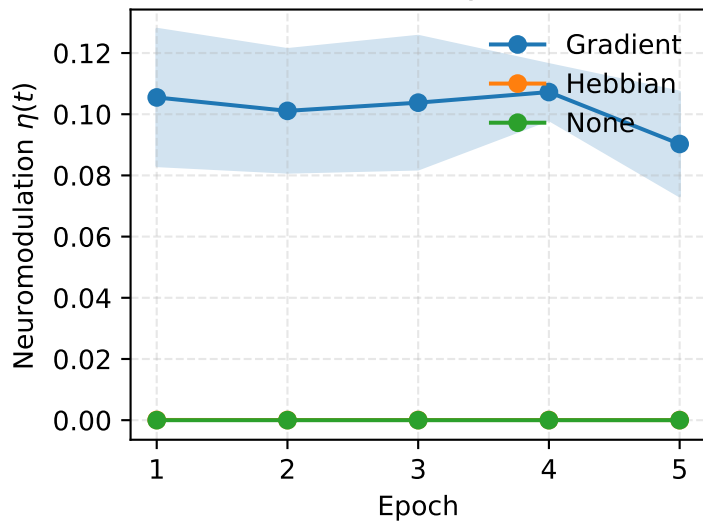
CIFAR-FS 5-way/1-shot
