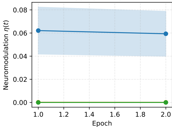
Copying (delay 20)
