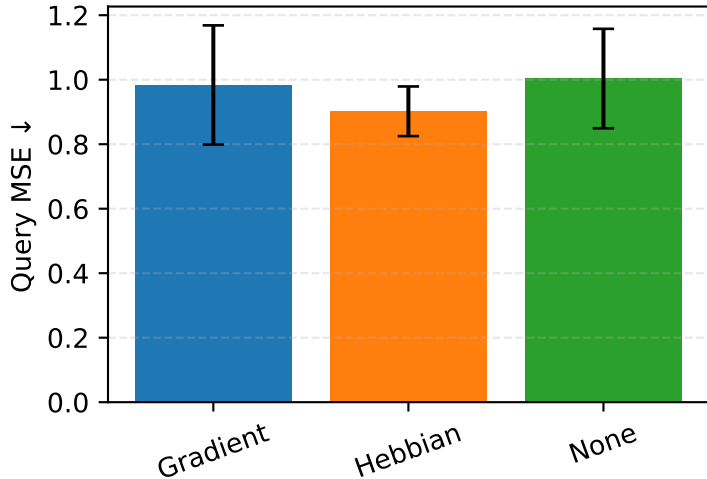
Few-Shot Regression (10-shot)
