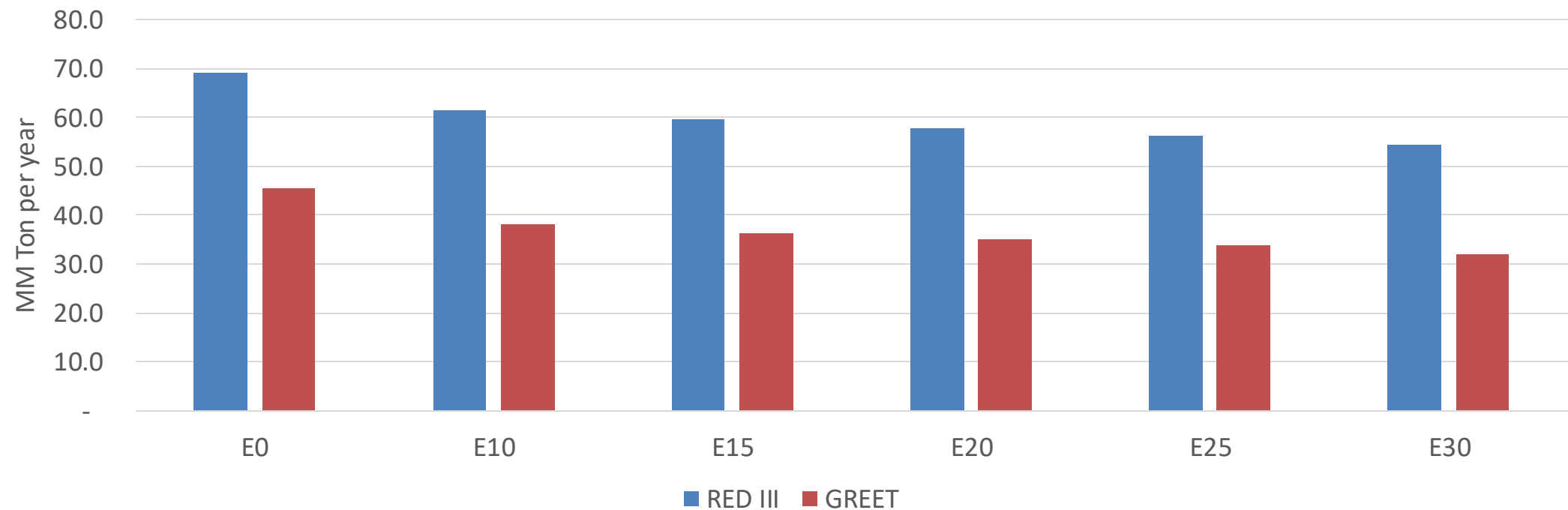
Life Cycle GHG Emission - Gasoline Vehicles
