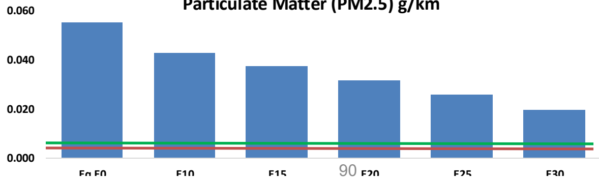
Particulate Matter (PM2.5) g/km
