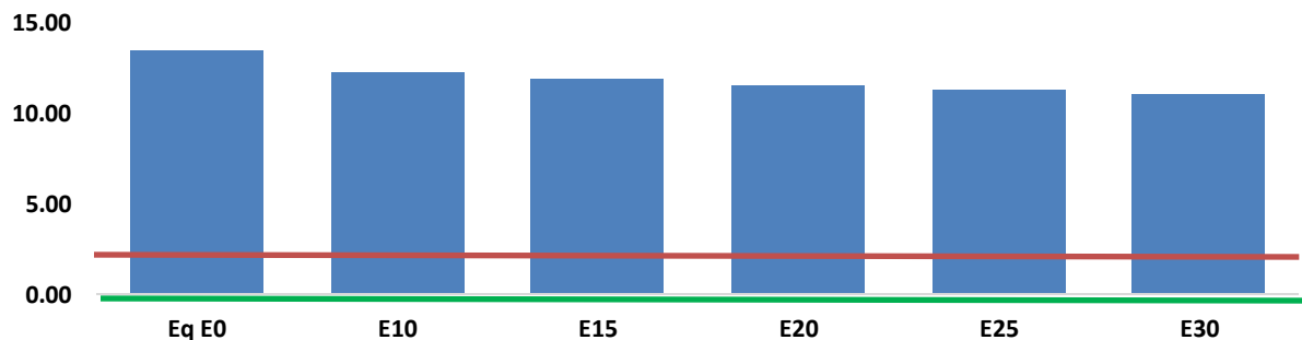
Carbon Monoxide (CO) g/km
