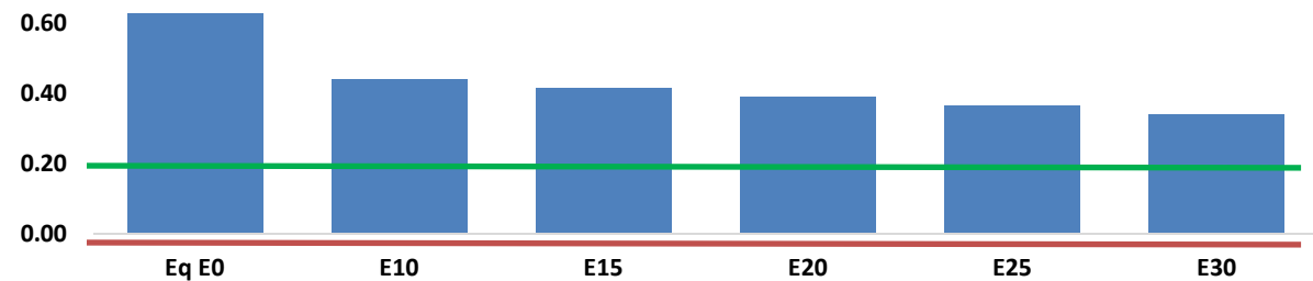
Nitrogen Oxides (NOx) g/km
