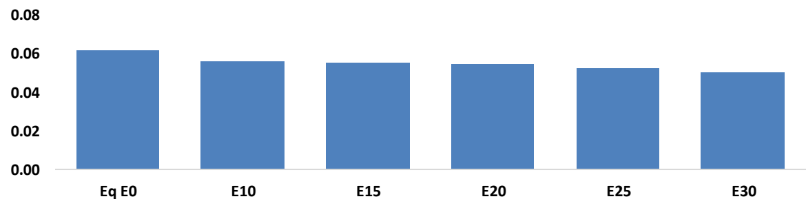
Aromatics (BTX) g/km
