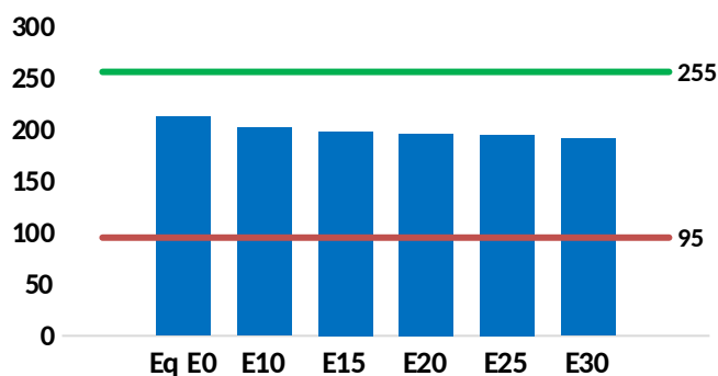
Carbon dioxide (CO2) in grams per km
