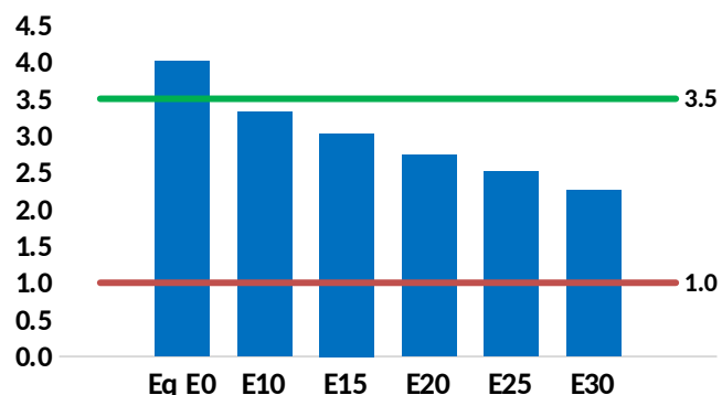
Carbon monoxide (CO) in grams per km
