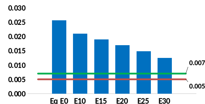
Particulated Matter (PM) in grams per km
