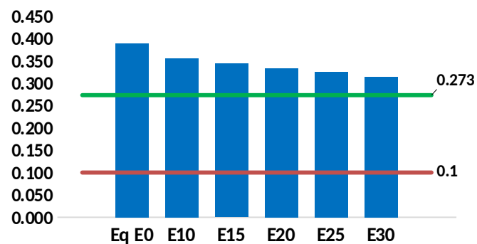
Total hydrocarbons (THC) in grams per km
