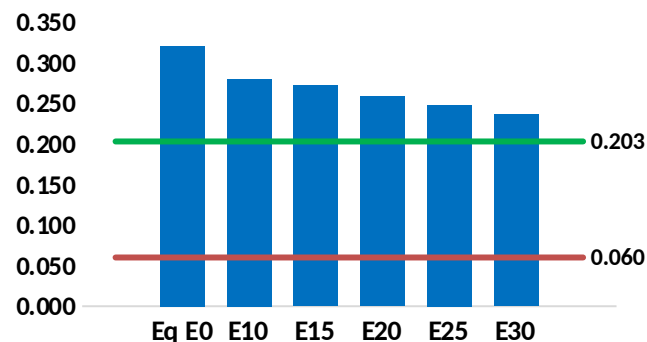
Nitrogen oxides (NOx) in grams per km
