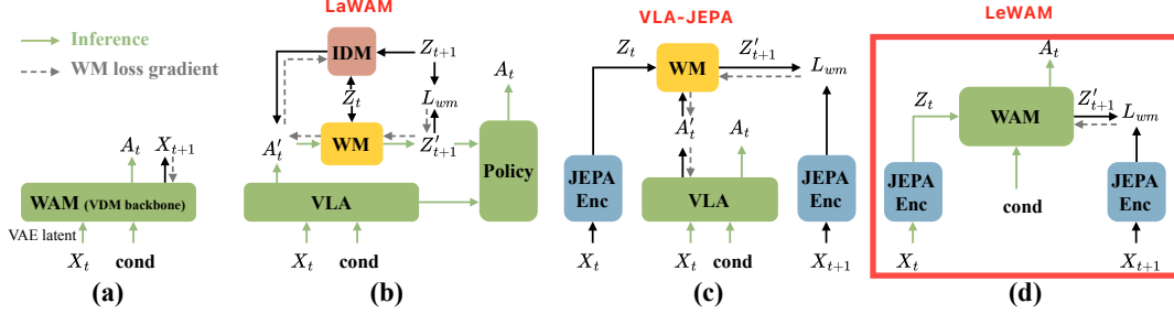
Figure 2: Comparison of WAM architectures. (a) Action-centered VDM-based WAMs use compressed VAE latents as visual inputs and jointly learn action generation and future frame prediction, but generate only actions at inference. (b) LaWAM (Chen et al., 2026) predicts latent actions from VLM representations and uses a separate world model to predict future DINOv3 embeddings, which condition action generation at inference. (c) VLA-JEPA (Sun et al., 2026) generates actions from VLM representations and uses latent action tokens to condition a separate world model supervised by V-JEPA2 embeddings during training. (d) LeWAM uses frozen I-JEPA embeddings as both visual inputs for action generation and targets for action-conditioned future prediction, learning both tasks with a single predictor while generating only actions at inference.
