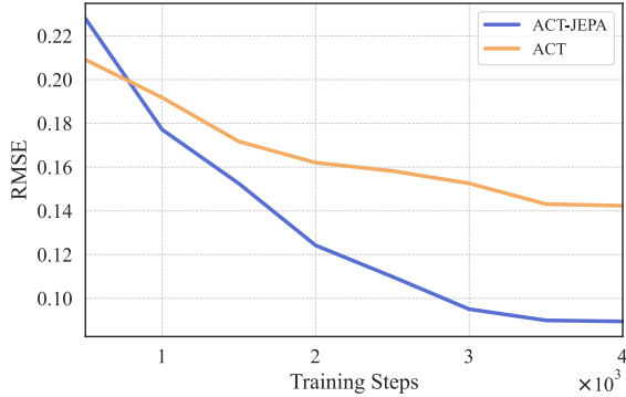
(a) ManiSkill RMSE ↓
