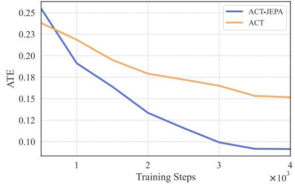
(b) ManiSkill ATE ↓
