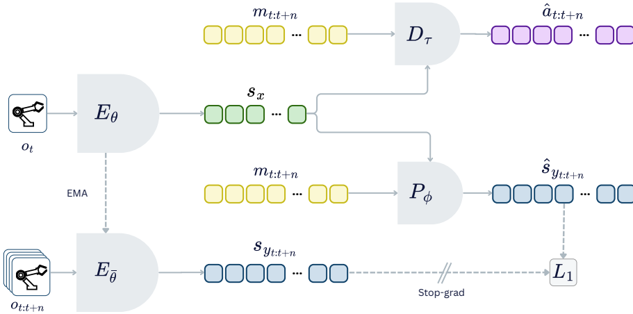
Figure 1: ACT-JEPA overview . The model is trained end-to-end to predict action sequences and latent observation sequences, with both objectives optimized using L_1 loss. It consists of four transformer-based components. The context encoder E_\theta encodes the current observation o_t into a latent representation s_x . The target encoder E_{\bar{\theta}} encodes future observations o_{t:t+n} into target latent representations s_{y_{t:t+n}} . Then, the predictor P_\phi takes s_x and learnable mask tokens to predict target latent representations \hat{s}_{y_{t:t+n}} . Finally, the new action decoder D_\tau takes s_x and learnable mask tokens to generate a sequence of actions \hat{a}_{t:t+n} . During inference, only E_\theta and D_\tau are utilized.
