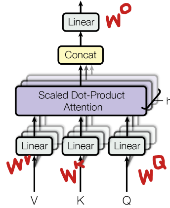
Multi-Head Attention
