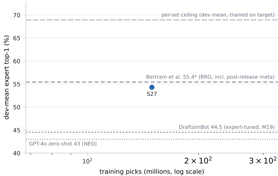
Figure 1: Zero-shot dev-trio-mean expert top-1 vs training picks (log scale). Filled points: the nested scaling ladder; open points: set-composition probes. Horizontal rules: published anchors and the per-set ceiling mean. Generated from run records by figures/scaling_curve.py ; rungs appear as their frozen evaluations land.
