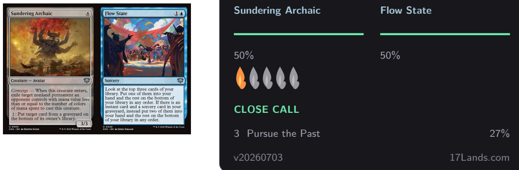
Figure 5: The low-conviction end of the same interface: a real thirteen-card SOS pack (empty pool) where the model’s top two EVs are (1.41 vs. 1.41) a near-exact tie, so the panel switches to a head-to-head duo view (§4.2) instead of naming a single pick. Dominance this close (50/50) is the regime top-label ECE below is measuring: the model’s stated confidence and its actual reliability at low conviction. Computed by the deployed per-set model, never MSH.
