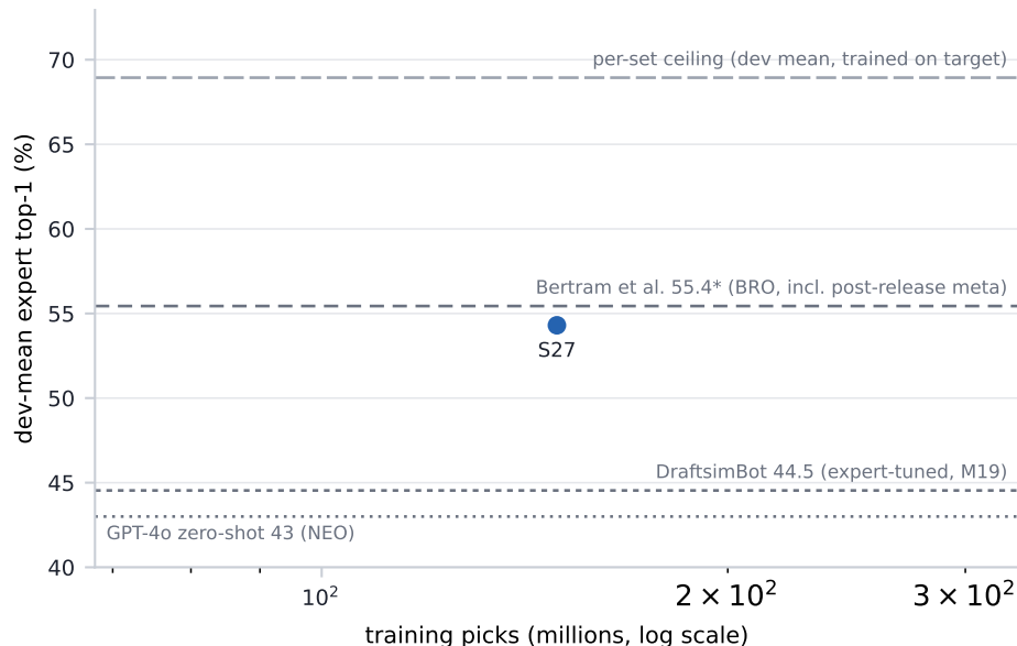
Figure 4: Zero-shot dev-trio-mean expert top-1 vs training picks (log scale). Filled points: the nested scaling ladder; open points: set-composition probes. Horizontal rules: published anchors and the per-set ceiling mean. Generated from run records by figures/scaling_curve.py ; rungs appear as their frozen evaluations land.
