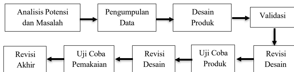
Gambar 1: Langkah-Langkah Penelitian
