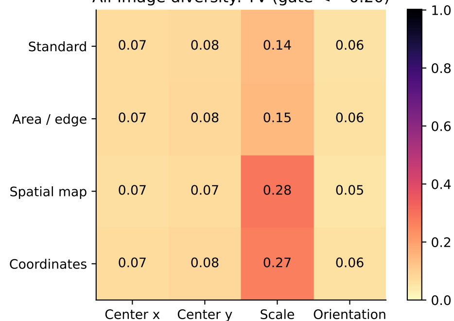
All-image diversity: TV (gate \leq 0.20 )
