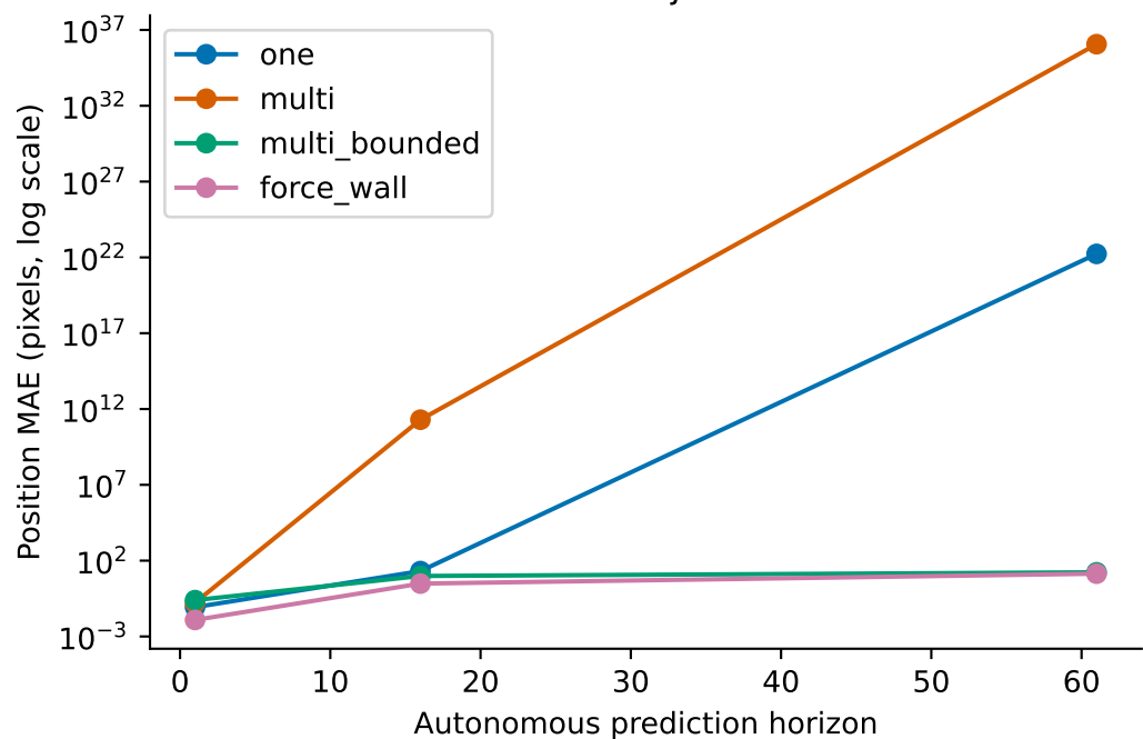
rgb_measurement
