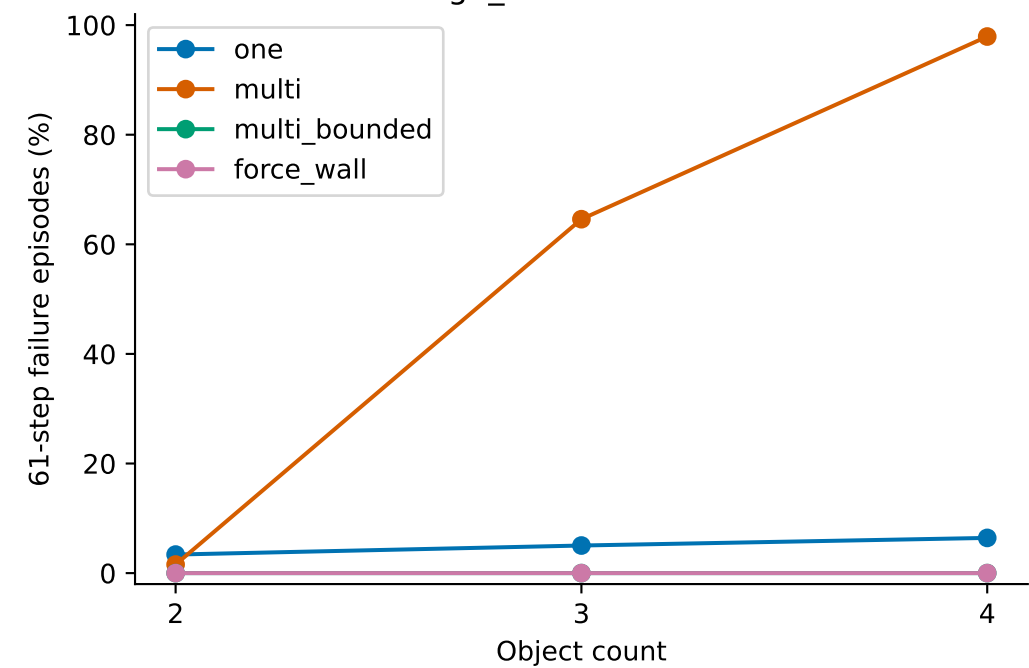
rgb_measurement
