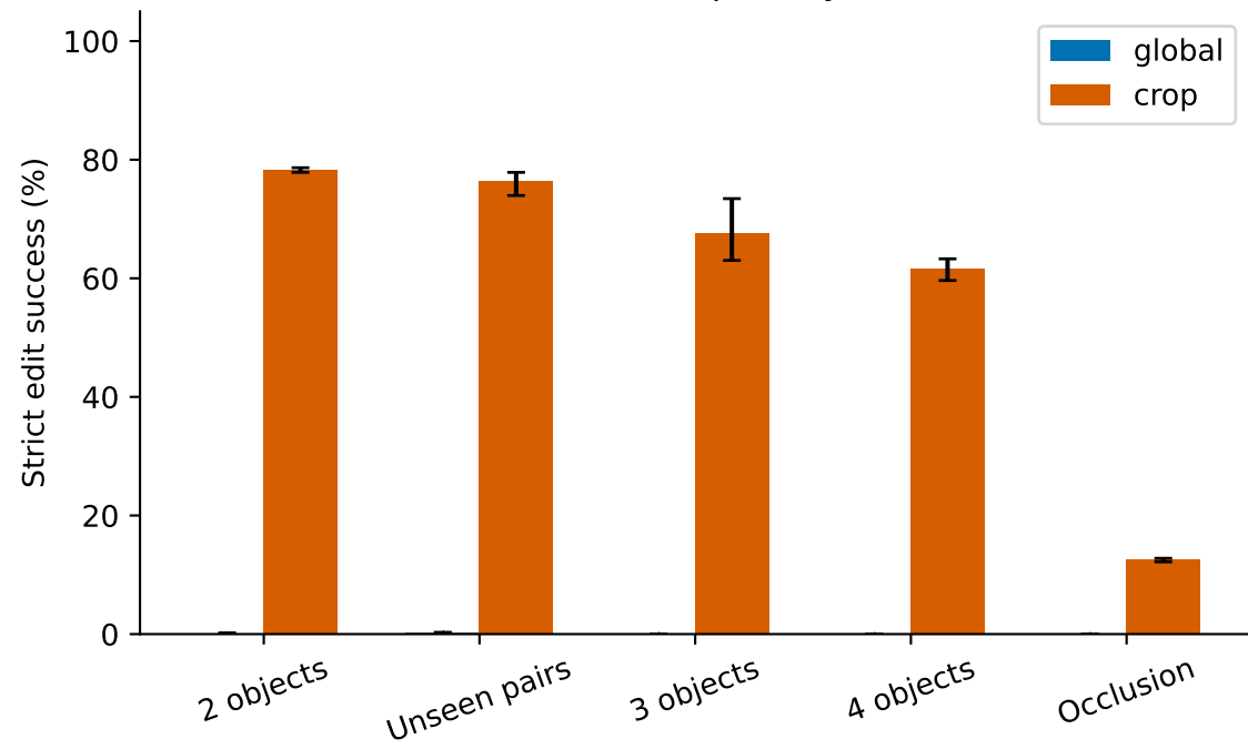
Initial crop study
