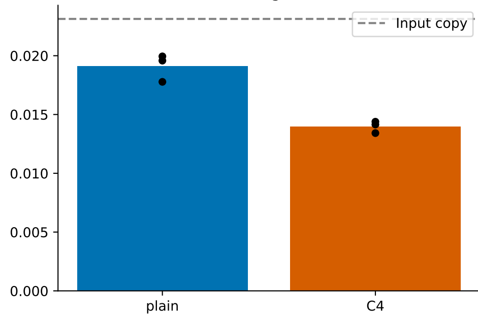
Full-image MSE
